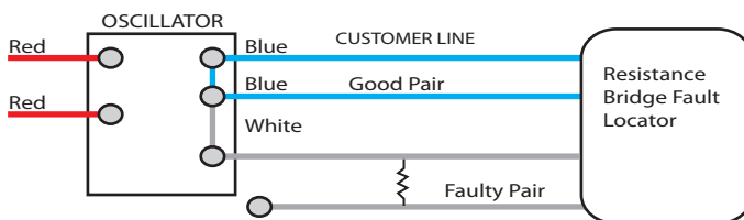
Figure 5 - 2 Three Wire Test
